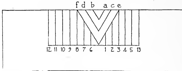
FIG. 263. ORDER FOR CHISELING OUT MORTISE.
